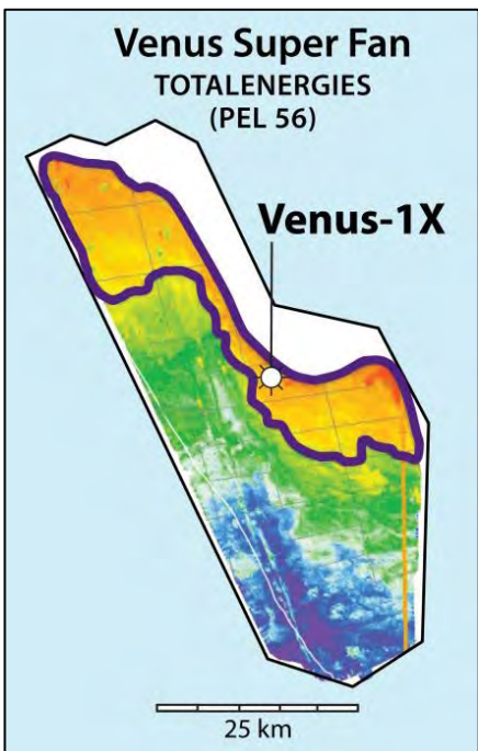
Orange Basin
