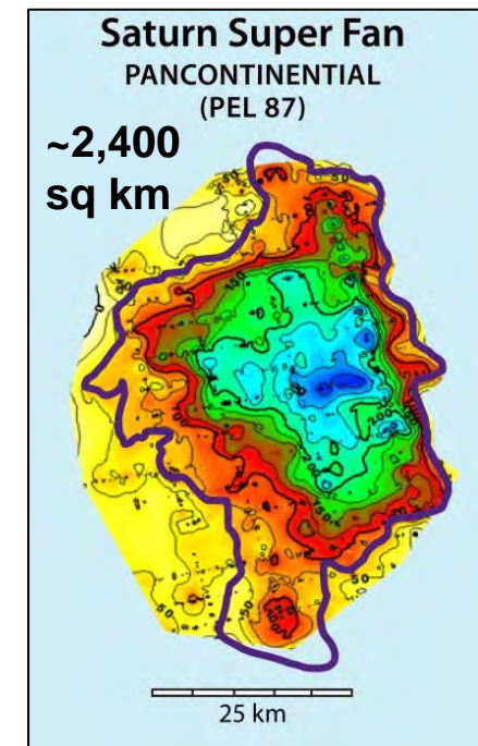
Orange Basin
