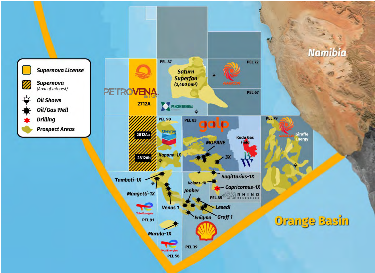
Orange Basin
